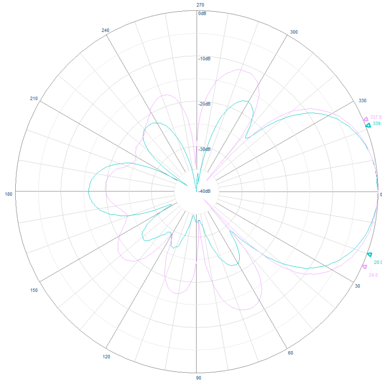
Example radiation pattern - Y806A-R
